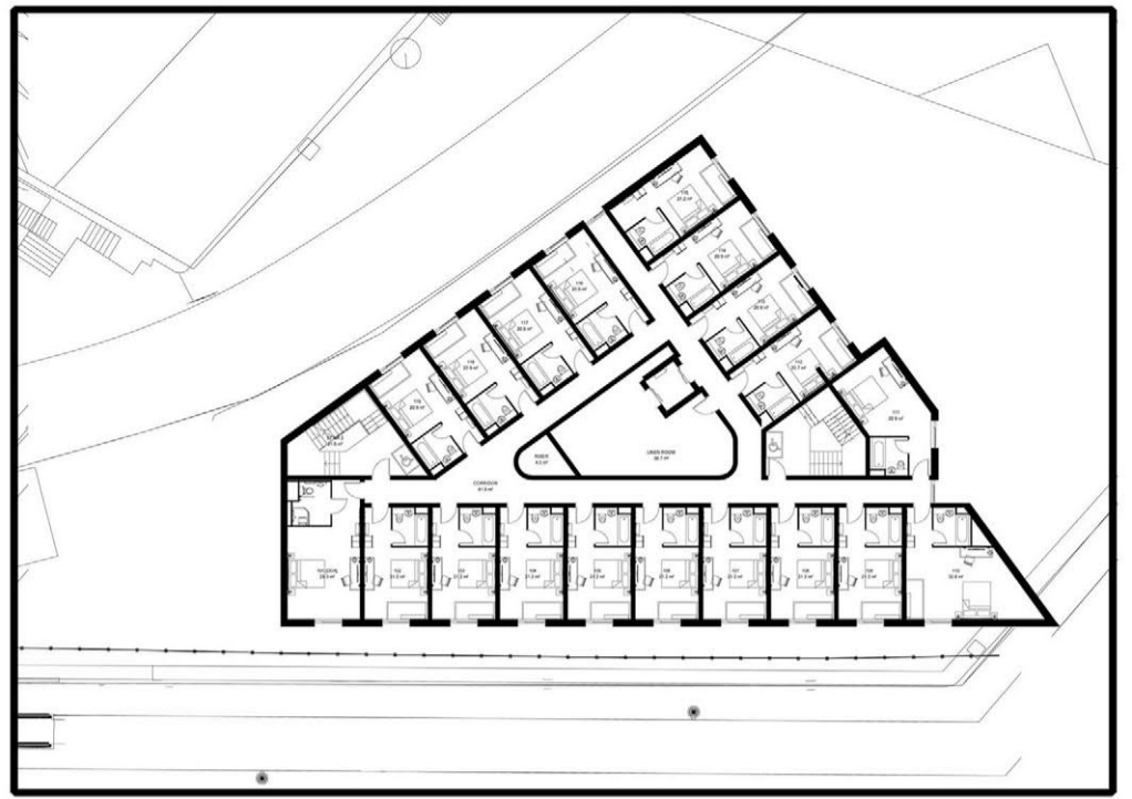
TYPICAL UPPER FLOOR PLAN
